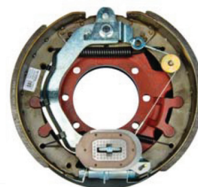
12K/16K, 12 1/4" x 5"
