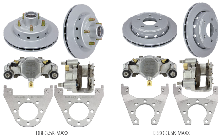
DBI-3.5K-MAXX
