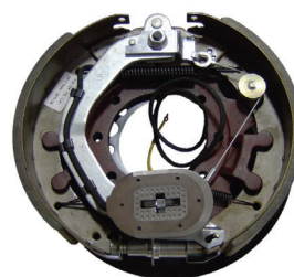
10K, 12 1/4" x 3 3/8"
