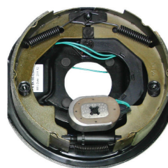
10" x 2 1/4"
