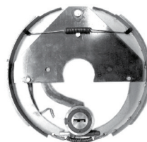
Electric Brake
